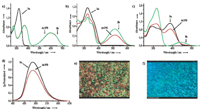
Figure 1. Absorption spectral changes of 1 (a), 2 (b), and 3 (c) and emission spectral changes of 3 (d) in cyclohexane solutions ( 2.05 \times 10^{-5} \text{ mol L}^{-1} ). Polarizing optical micrograph of 1 , supercooled to room temperature, before irradiation (e) and after irradiation (f) of 1 min with 366 nm light.
